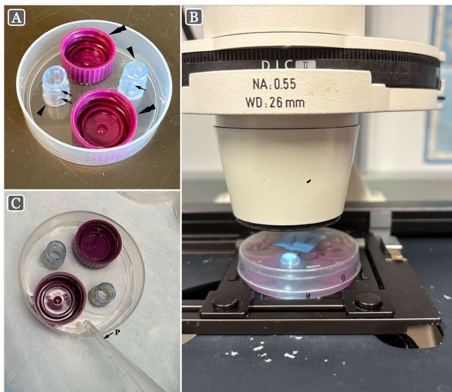
FIGURE 1 | Preparation of single cells for transmission electron microscopy (TEM) using TEM fixation plates. (A) General structure of the TEM plates used for single-cell preparation. Baskets constructed from 1000 µL pipette tips (arrowheads) are affixed to the base of a polypropylene Petri dish using waterproof silicone sealant. Holes made in baskets that facilitate liquid exchange are shown (arrows). Lids from 15 mL Falcon tubes (double arrowheads) are placed inside the dish to reduce its internal volume, allowing smaller volumes of waste associated with fixatives and buffers used during processing. (B) Fixatives and buffers can be added and removed from TEM plates containing single cells using a plastic transfer pipette (P). Liquids should be added and removed from outside of each basket to avoid disturbing or resuspending cells. (C) Cells can be visualized at any point during the sample preparation process using an inverted light microscope, except during steps when a fume hood is recommended.
