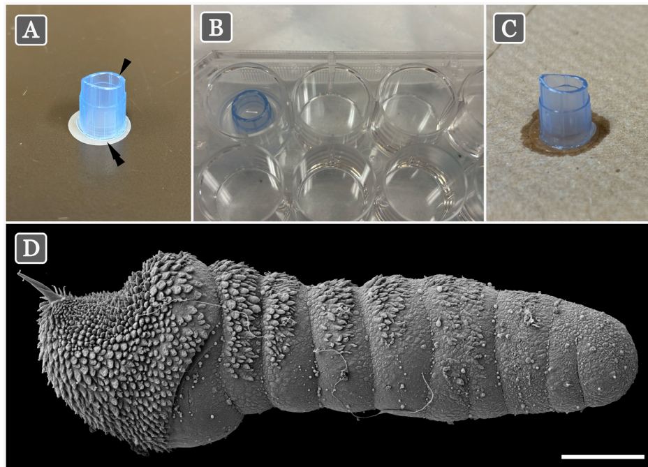
FIGURE 4 | Preparation of single cells for scanning electron microscopy (SEM) using custom-made baskets. (A) SEM preparation basket constructed from the blunt end of a 1000 µL pipette attached to a 5 µm isopore membrane filter using silicone. (B) An SEM basket containing fixed cells inside of a 24-well plate during a washing step. The basket and the well are both filled ~50% of the way with filtered sea water. (C) SEM baskets containing fixed cells are placed on a piece of paper towel to facilitate liquid exchange. Fresh reagent (depending on the step of SEM processing) is placed directly inside of the basket as it is drained to ensure cells are never exposed to air. (D) A single parasite of Haplozoon sp. (Dinoflagellata) prepared using this approach for SEM. Scale bar = 10 µm.
