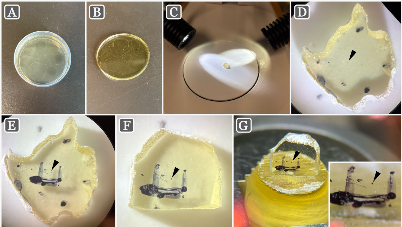
FIGURE 2 | Preparing flat-embedded single cells for ultramicrotomy. (A and B) Cells are flat embedded within the Petri dish used for fixation and dehydration upon the removal of baskets and falcon tube lids. The resulting polymerized resin puck can be scanned for fixed cells using an inverted light microscope or stereoscope. The position of cells within the resin is marked using a fine-tip marker. (C–E) The resin containing the cell of interest can be excised from the larger resin block using a Dremel tool. Guiding lines are then drawn around the embedded cell to aid in precise orientation. Two lines are marked parallel to the cell's x - y axis, and a third line is drawn perpendicular to the cell. (F) The edges of the resin block are polished using a Dremel tool, following the guiding lines drawn around the cell of interest. The base of the block (the surface to be adhered to the empty resin block) is trimmed to be parallel to the lower horizontal guiding line to ensure proper orientation for ultramicrotomy. (G) The prepared resin block containing the cell of interest is mounted on an empty resin block and can be observed using an ultramicrotome. Inset: High magnification view of the cell contained within the resin block, ready to be trimmed and faced for ultramicrotome sectioning.
